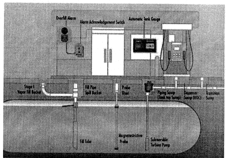
Typical Installation
