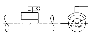
Saddle
