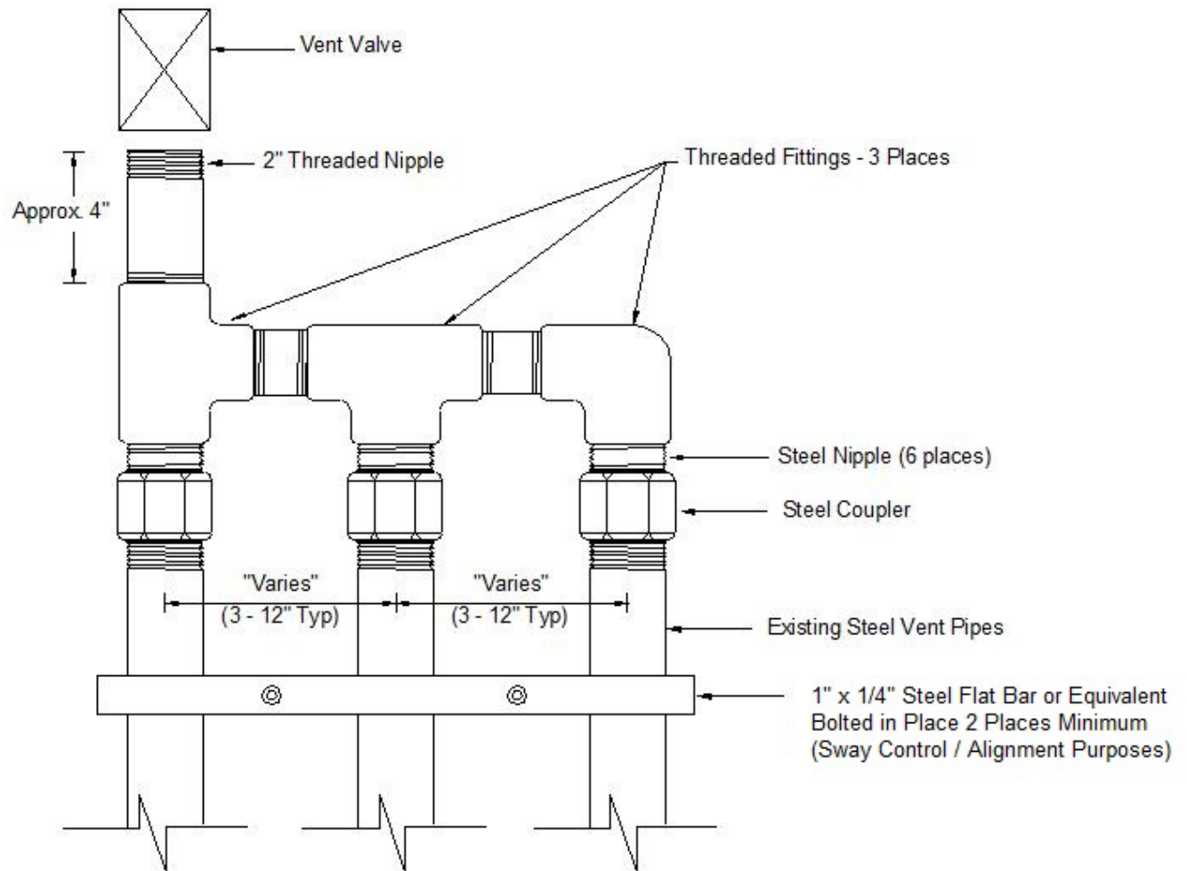
Figure 2-7 Typical Vent Pipe Manifold
