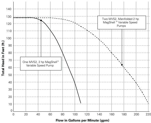
2 Hp Variable Speed Pump Performance Chart
