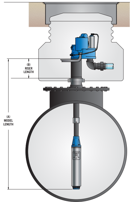
Model Length (A)
