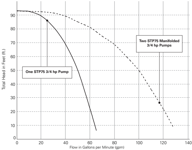
¾ Hp Fixed Speed Pump Performance Chart
